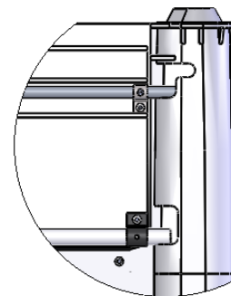
DETAIL B SCALE 1 : 10
